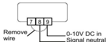
Figure 8: Wiring of external control signal
