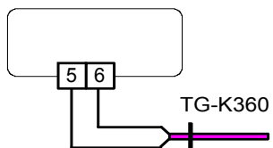
Figure 7: Wiring of a limitation sensor
