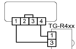
Figure 3: Wiring of TG-R430 sensor as external sensor and setpoint adjustment for room control
