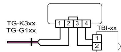
Figure 6: Wiring of an external, separate sensor and a TBI-xx potentiometer as a setpoint device
