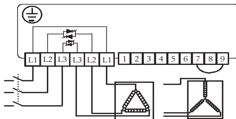
Figure 1: Wiring of supply voltage and load
