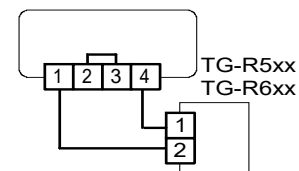
Figure 2: Wiring of room temperature sensor TG-R5xx or TG-R6xx when using internal setpoint
