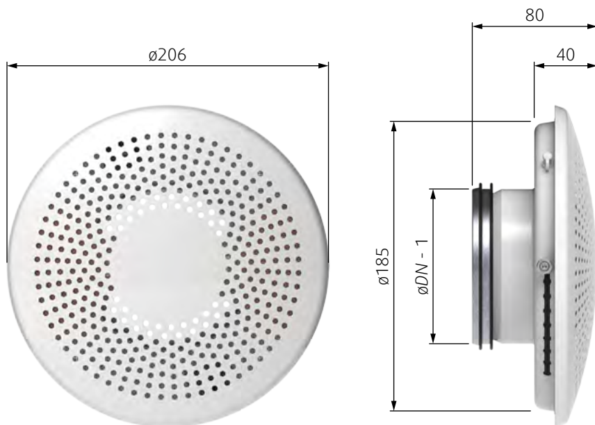
Fig. 2: Dimensions of the BOR-R
