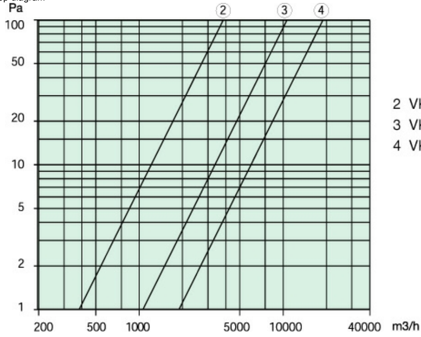
Pressure drop diagram
