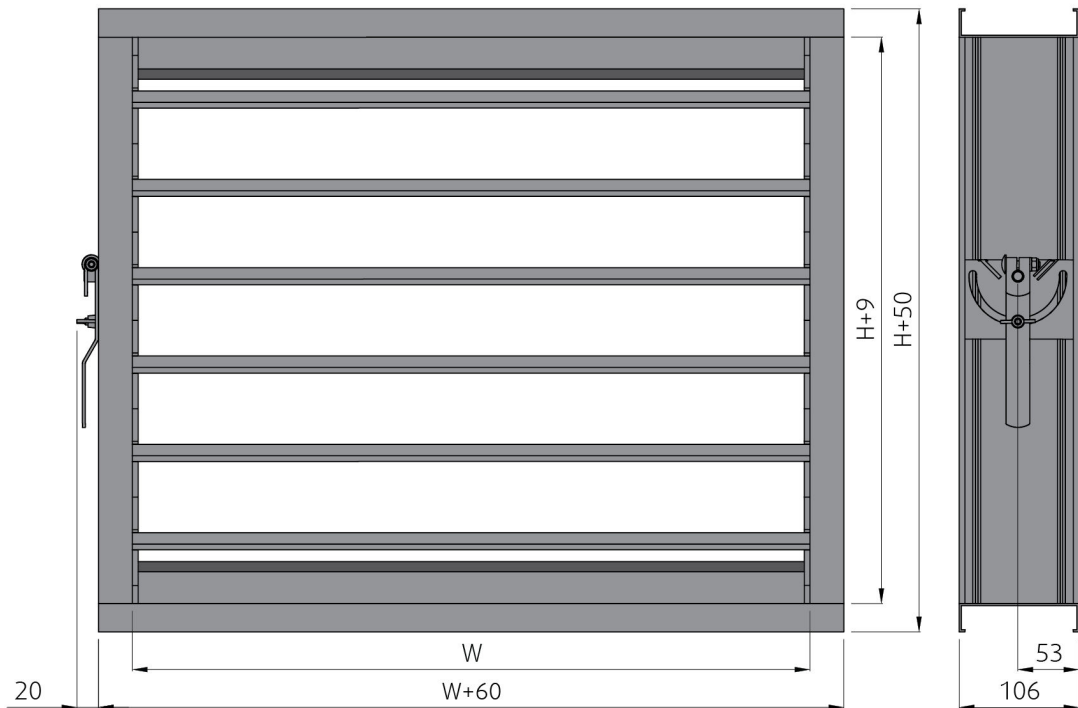
Dimensions of RK-WxH-R and RKT-WxH-R - manual version
