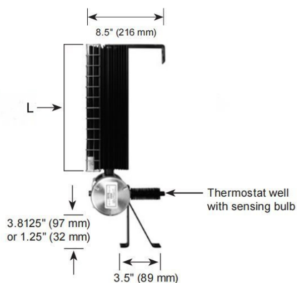
KX floor mounted
