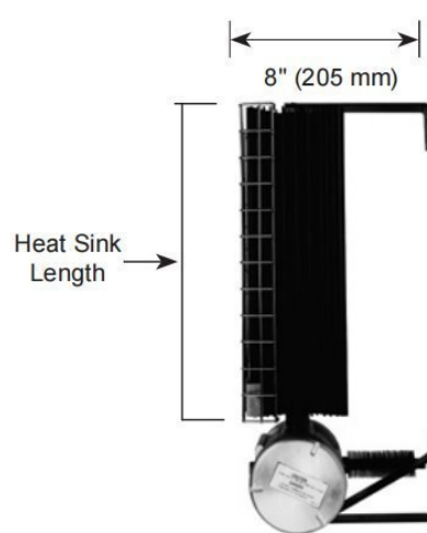
KX wall mounted
