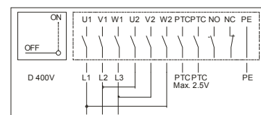
WD6: wiring D; single speed motor, with EMC protection all wires led out, for frequency converter use
