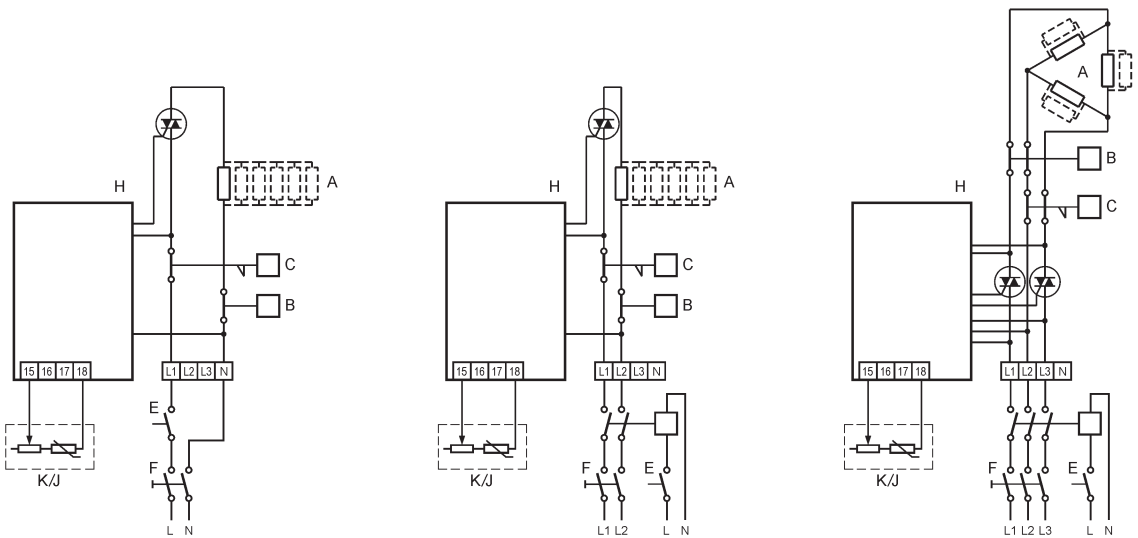
CBMF-1e (230V~)
